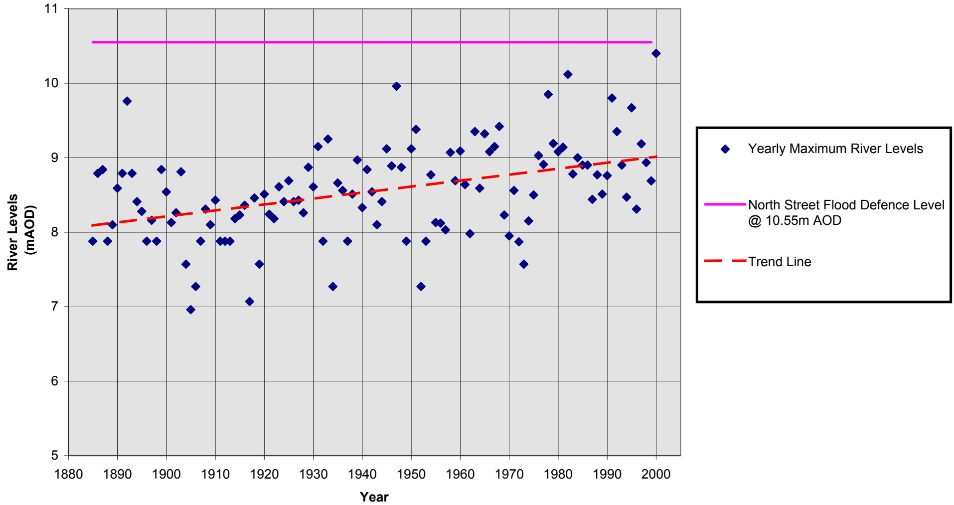
FIGURE 5 : River Ouse Yearly Maximum Flood Levels (@ Viking Recorder)
